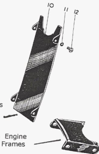
66.4181 Gen BSA ( used) BSA M20/21/33. Engine Plate Cover (front) Rigid and Spring Frames 1949/53 EURO 21.70.
